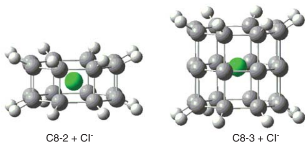
Figure 3. C8-2 and C8-3 structures as carriers of one chloride anion.
