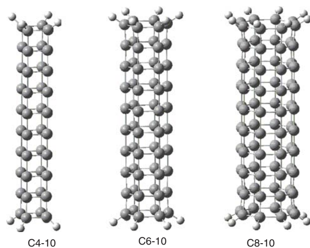
Figure 1. Structure of C4, C6 and C8 carbon nanoneedles with 4, 6 and 8 terminal units, respectively, and 10 layers.
