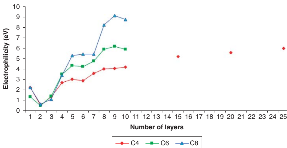
Figure 2. Electrophilicity versus number of layers for C4, C6 and C8 carbon nanoneedles.
